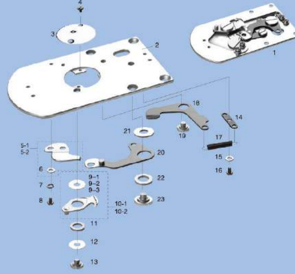
BE-438D 剪线组件 ASSEMBLY FOR BE-438D
