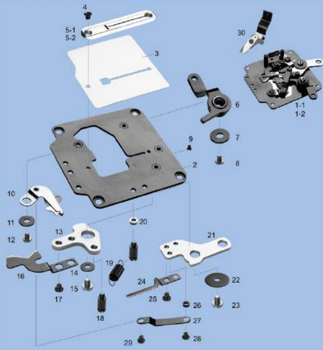
LBH-1790 剪线组 ASSEMBLY FOR LBH-1790
