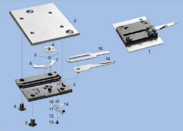
LZ-2290 剪线组件 ASSEMBLY FOR LZ-2290
